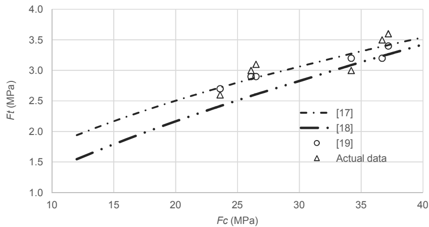
Fig. 5. Splitting tensile strength based on compressive strength
