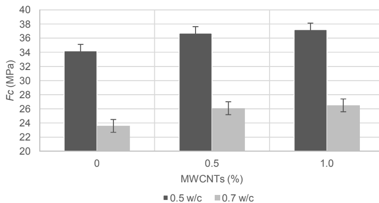
Fig. 2. Compressive strength based on MWCNTs and w/c
